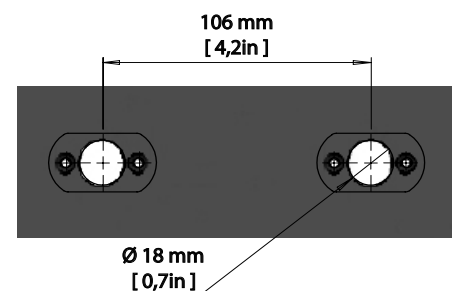
Figure 2: i-2 Series locking points
