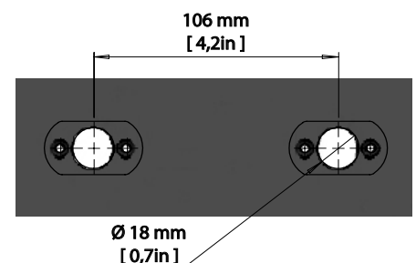
Figure 2: P-2 Series locking points
