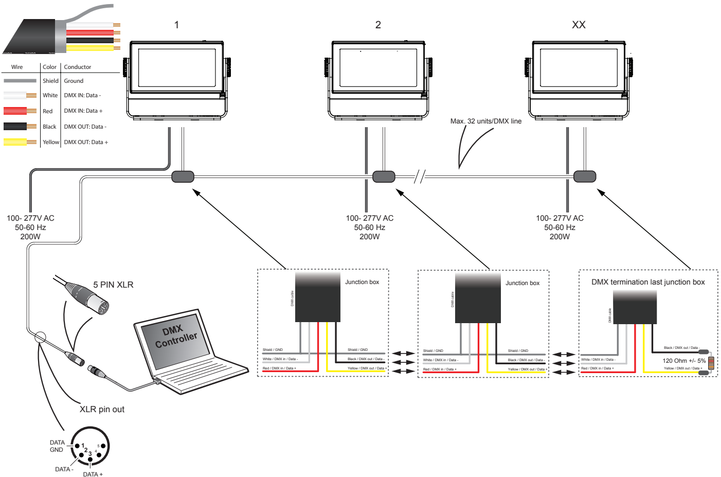
Figure 18: Connecting DMX and AC Power in P-2 POI
