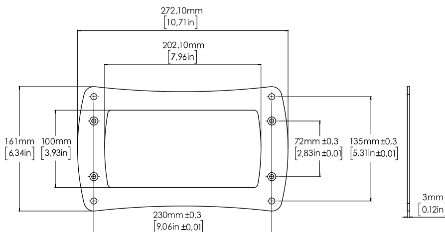
Figure 5: P-2 mounting bracket
