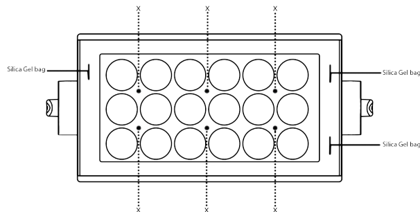
Figure 27: P-2 Changing lens module III
