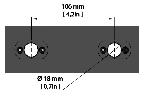
Figure 2: P-10 Series locking points
