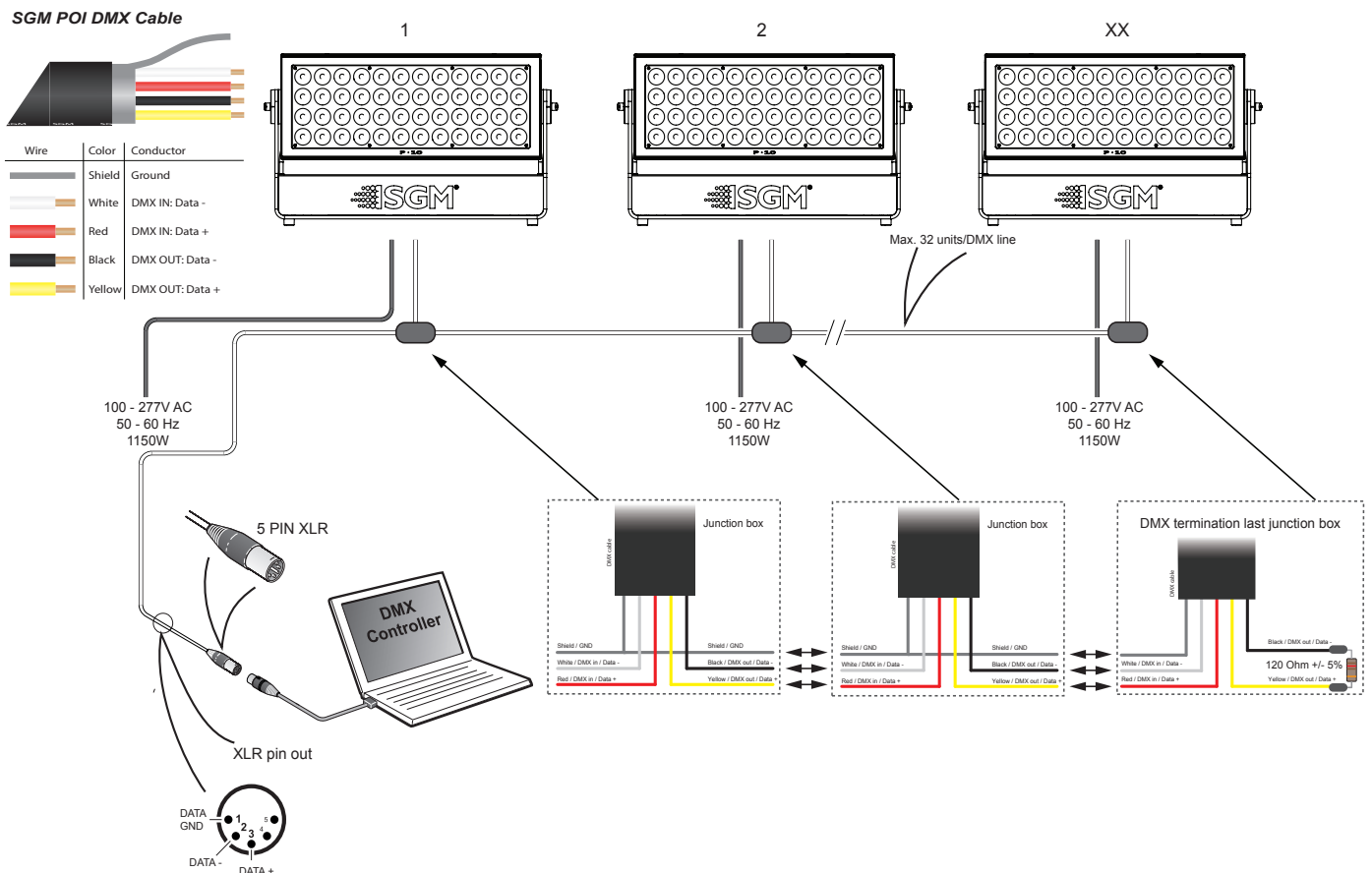
Figure 19: Connecting DMX and AC Power in P-10 POI
