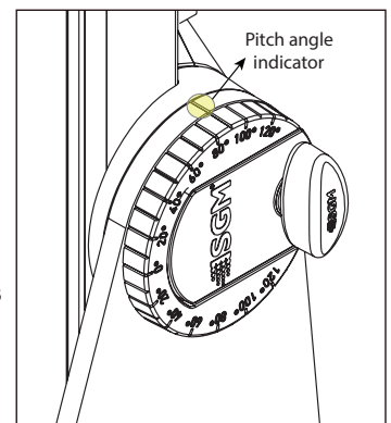
Figure 5: Tilt lock
