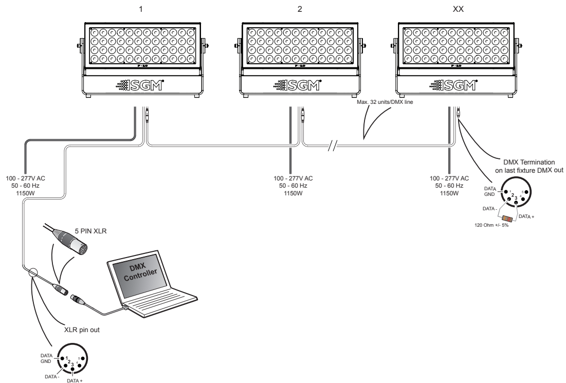
Figure 11: P-10 connection diagram (see page 17 for POI)
