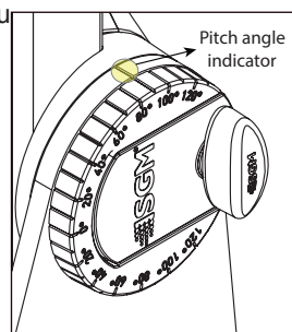
Figure 5: Tilt lock
