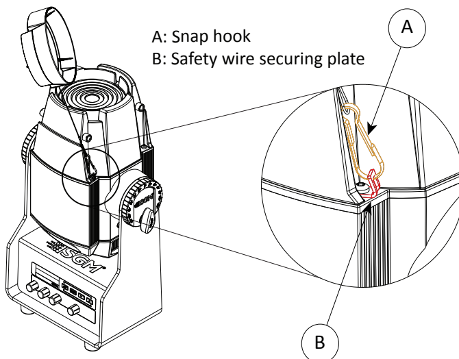
Figure 17: Attaching the Top Hat safety wire
