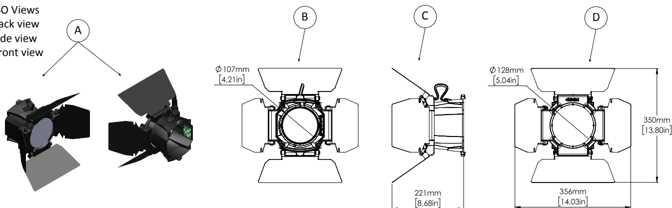
Figure 19: Motorized Barndoors front lens
