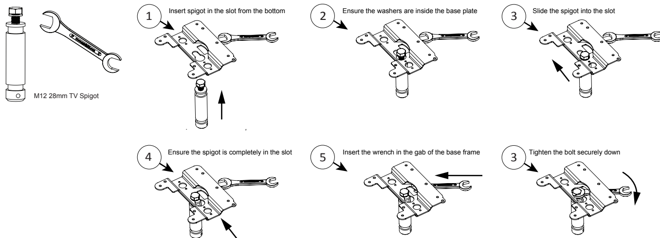
Figure 3: Spigot mounting
