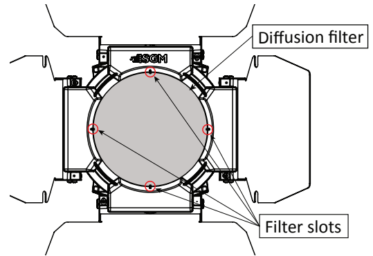
Figure 22: Diffusion filter and slots
