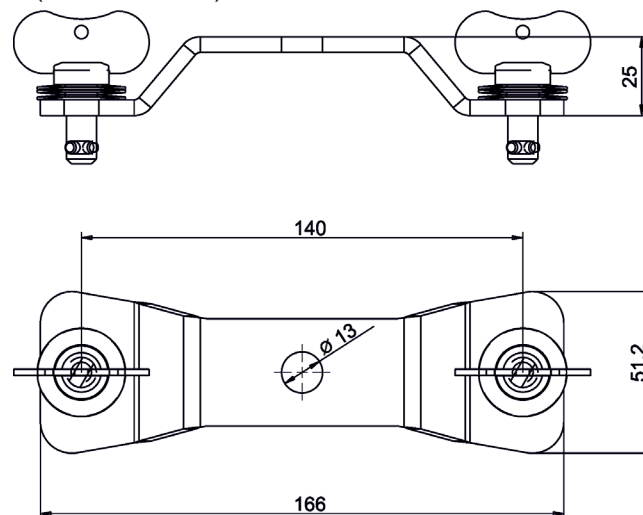
Omega adaptor CL-regular (P/N 10980033)
