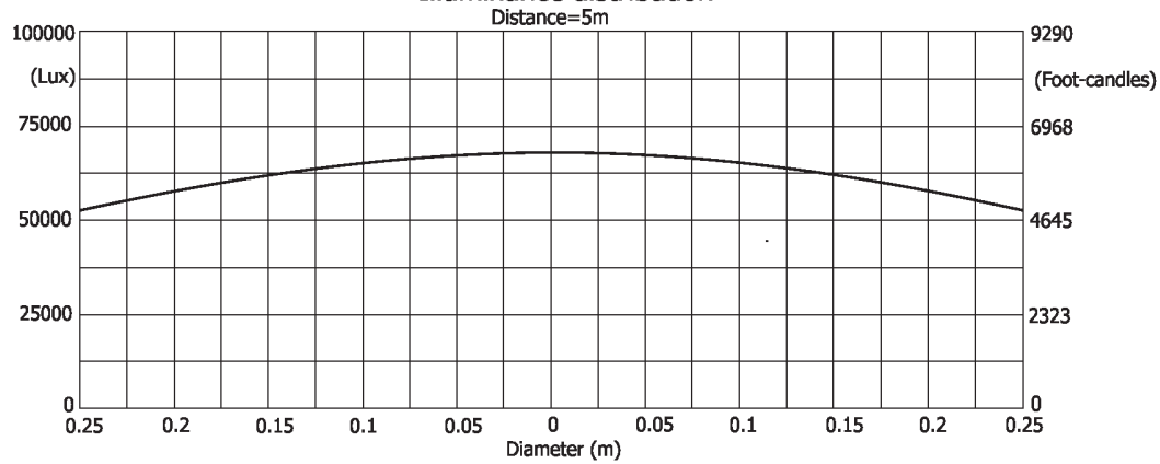
Illuminance distribution
